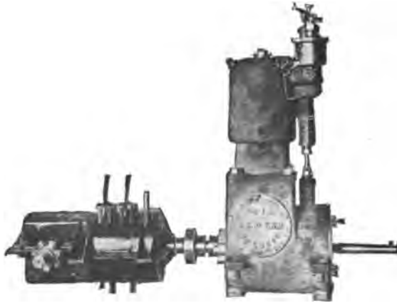
FIG. 416.—The "Dyke" Gasoline Carriage Motor, shown connected to the clutch transmission and change-speed gear.
